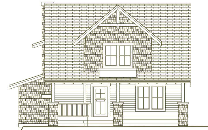
Front Elevation
